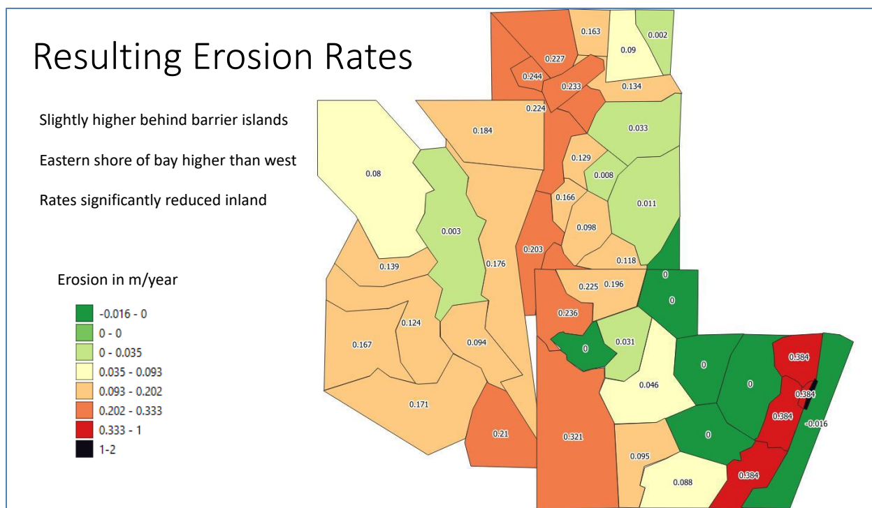
Figure 17. Resulting erosion rate polygon dataset.
