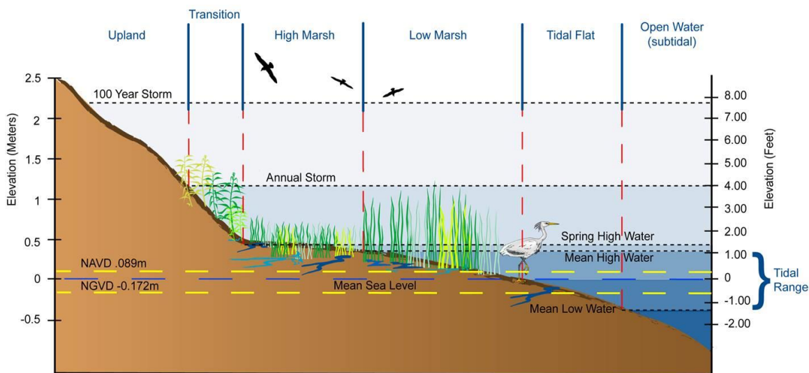
Figure 10. Relationship between tides, wetlands, and reference elevations for an example estuarine shore profile. Source (Titus and Wang 2008)
